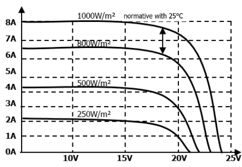
Production influence according to irradiance Ex. 150W solar panel
